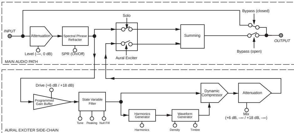
Block Diagram of Apex Aural Exciter, Type III
